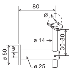
Handrail Wall Bracket
