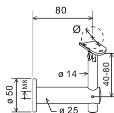
Adj.Handrail Wall Bracket
