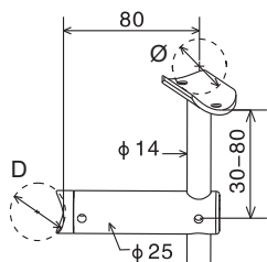
Handrail Tube Bracket
