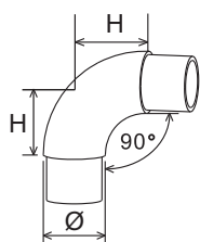
Flush Joiner 90 Degree Radiused
