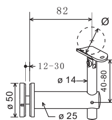
Adj.Handrail Glass Bracket
