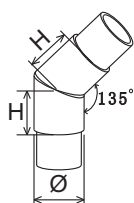
Flush Joiner 135 Degree
