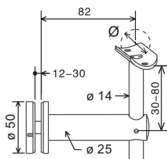
Handrail Glass Bracket
