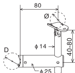
Adj.Handrail Tube Bracket
